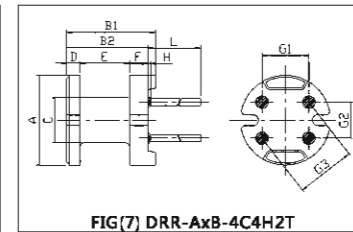
FIG(7) DRR-AxB-4C4H2T
