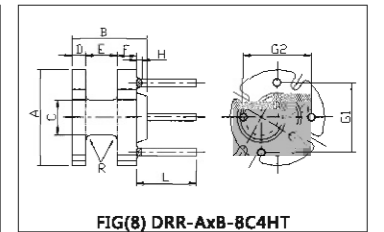
FIG(8) DRR-AxB-8C4HT
